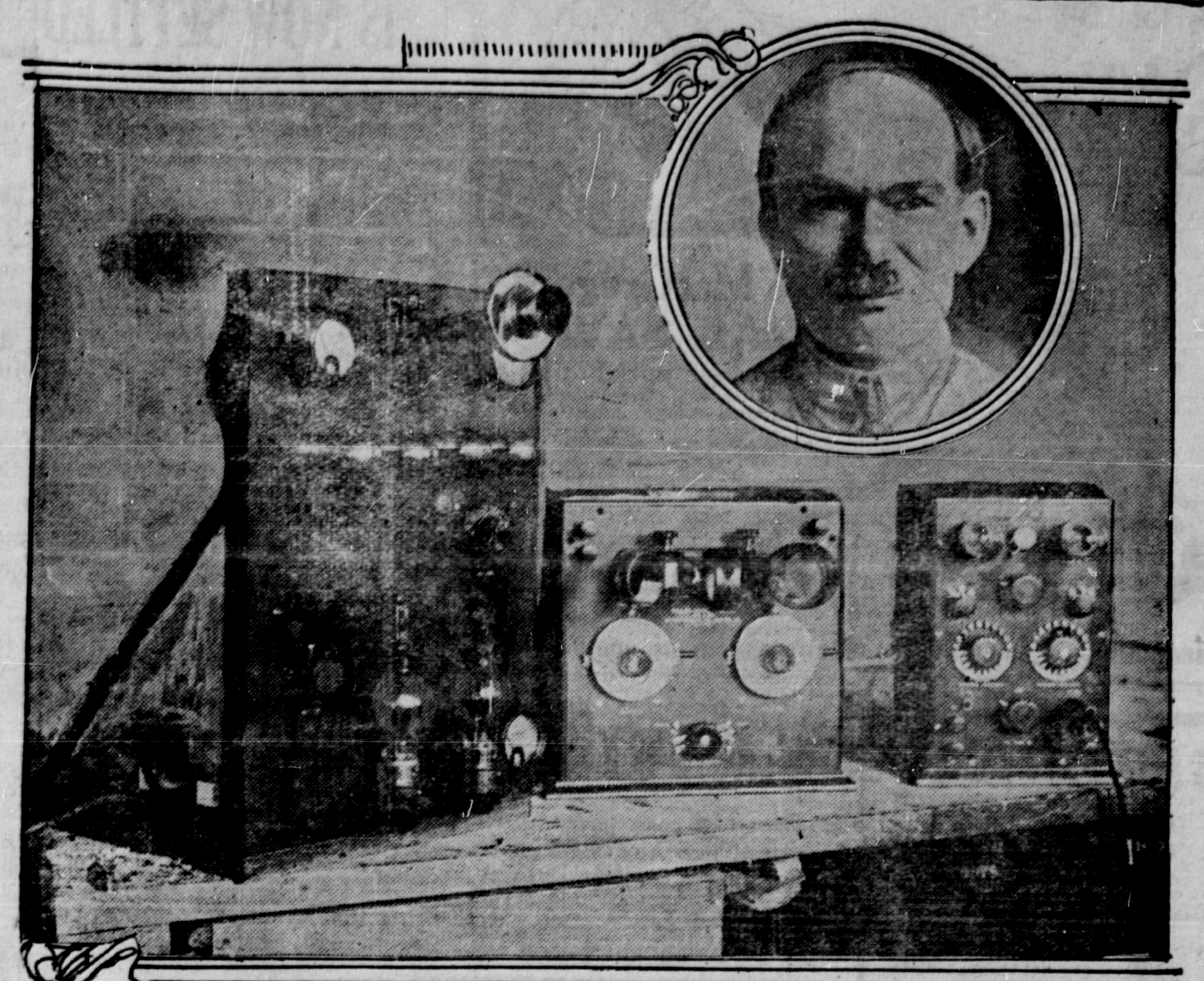
The complete outfit of the "baby wireless" telephone, showing the transmitter, the tuning set for locating calls and the receiving set. The inventor, D. Lee De Forest, says with this equipment it is possible to talk with the occupant of a moving automobile.
