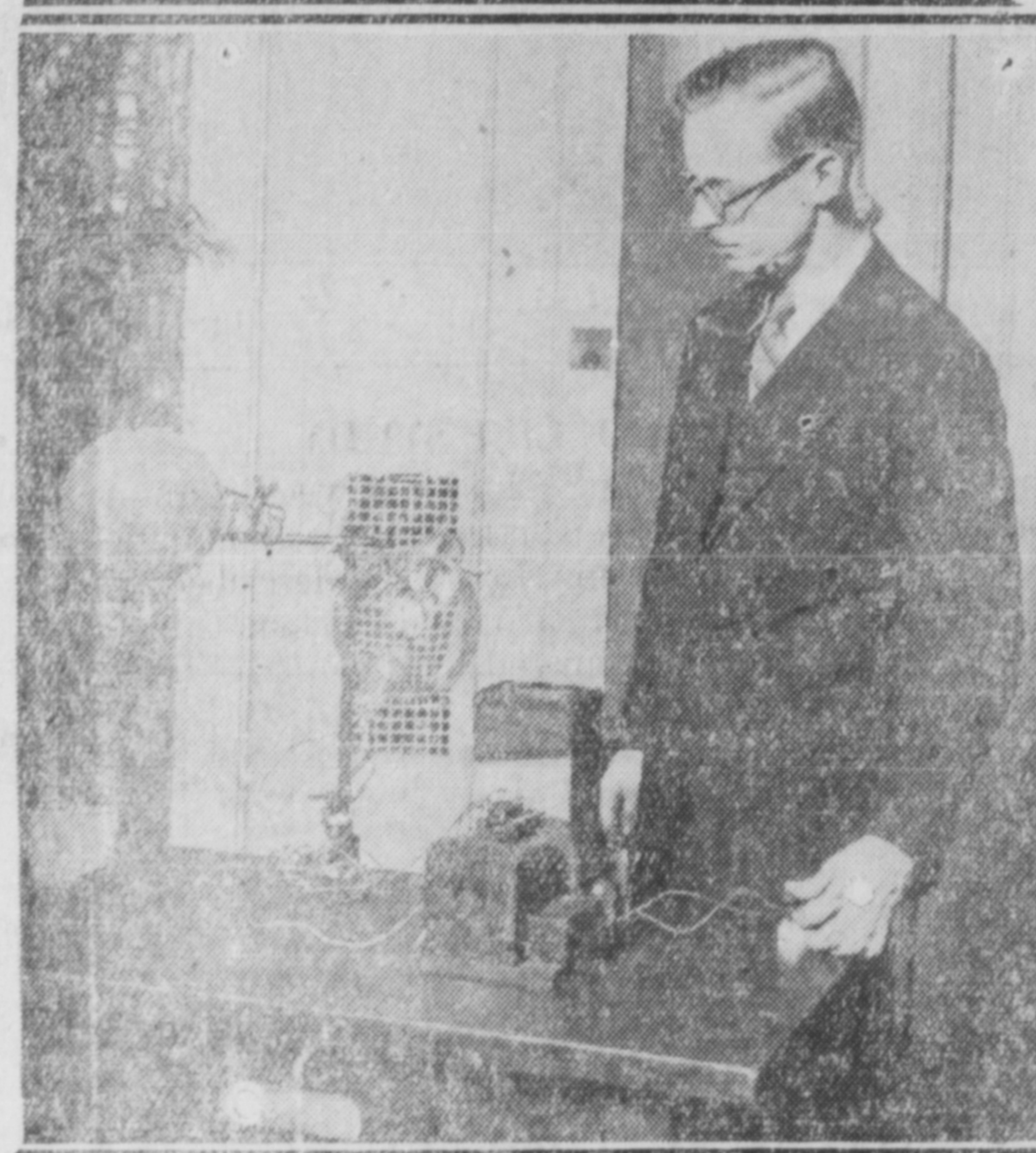
OBTAINS AN "AUTOGRAPH" OF LIGHTNING FLASH A. L. Atherton, electrical engineer, has devised an instrument for placing on record everything necessary for the analysis of lightning.
