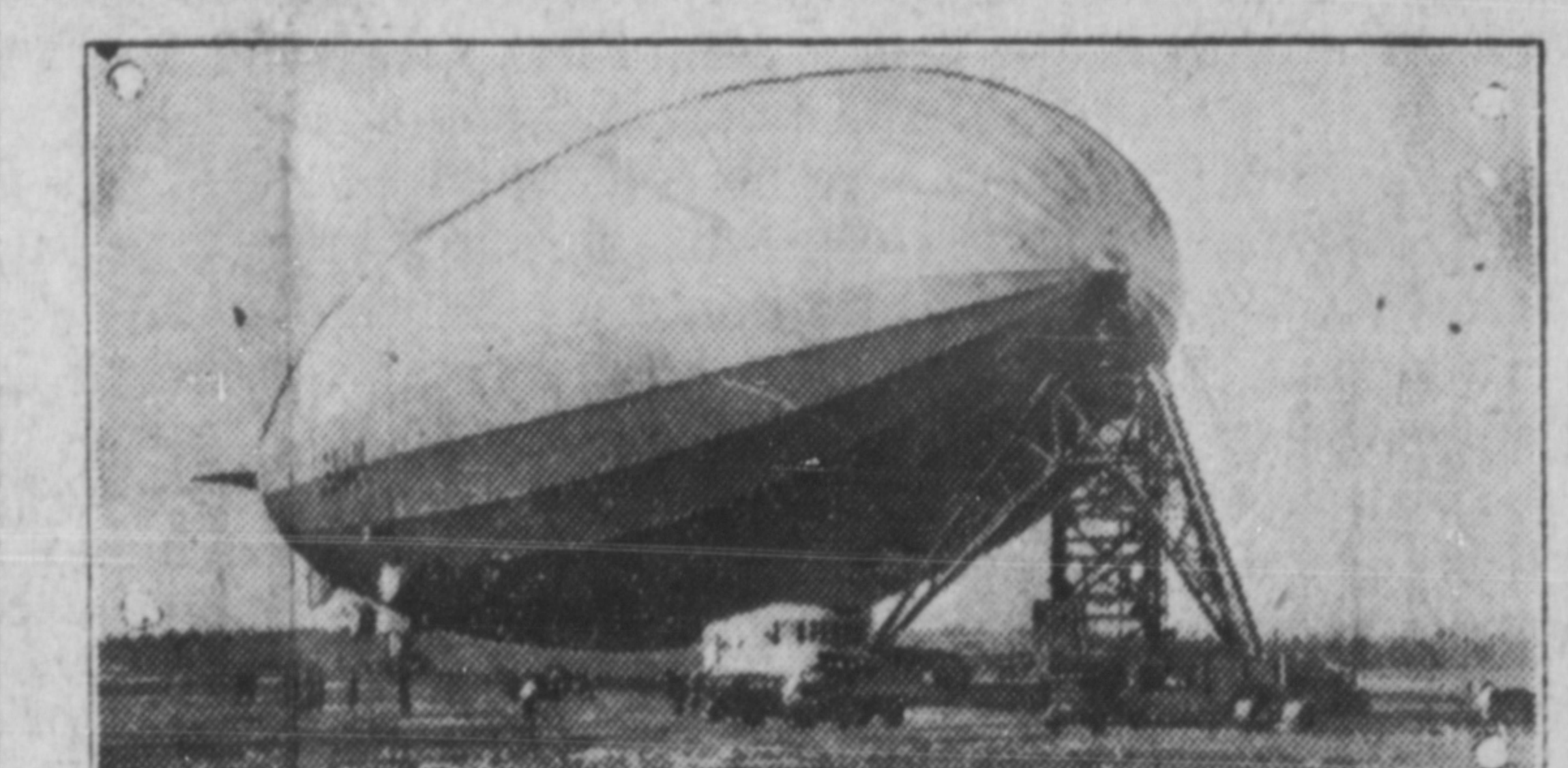
New type of mobile "stub" mooring mast used successfully at Lakehurst, N.J., naval air station. The Los Angeles is seen here moored to it.
