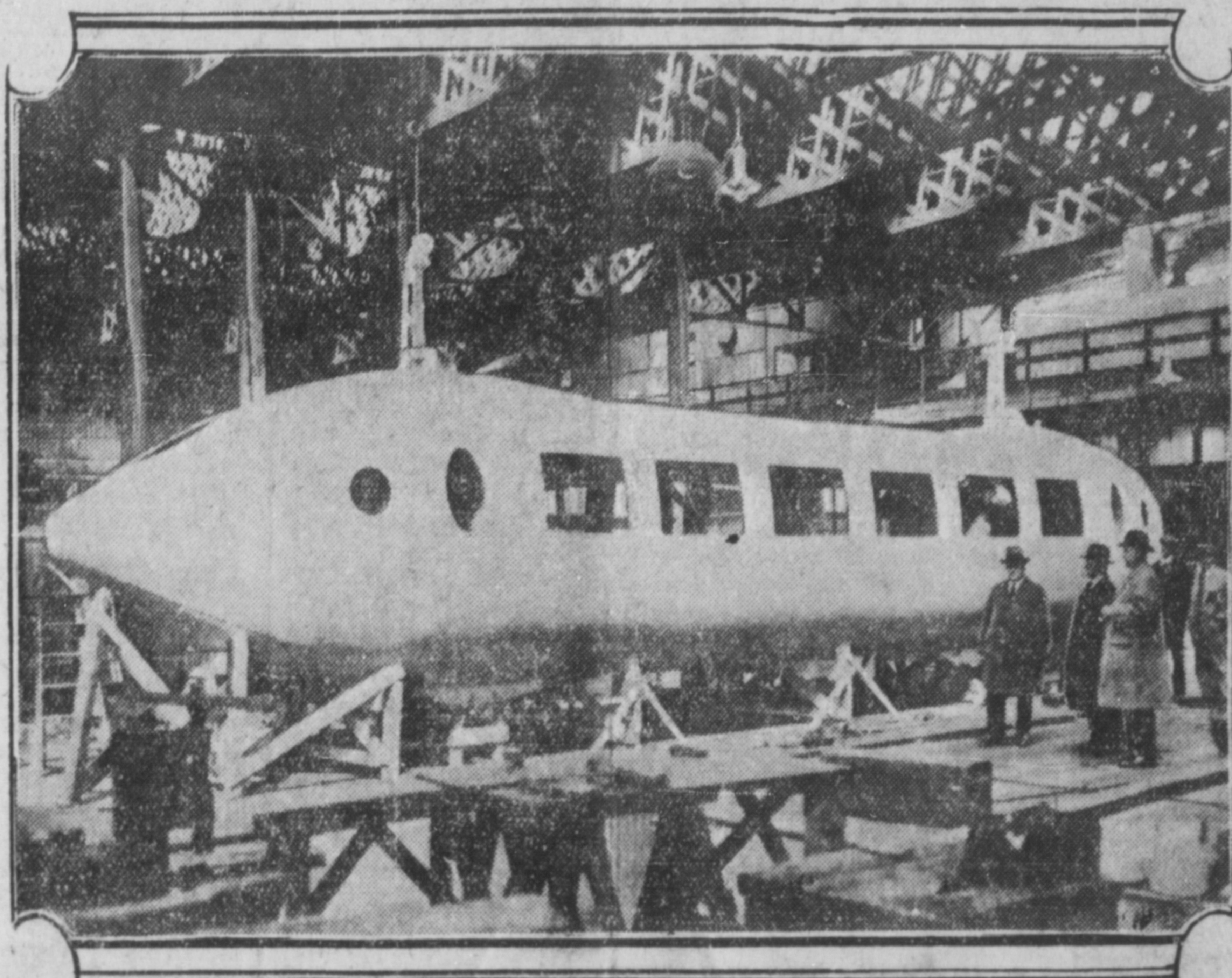
Remarkable system of new transport is to be tried out next month at Milngavie, near Glasgow, when the "rail plane," invented by Mr. George Bennie, will be demonstrated to the public. The coach-shaped like an airship, will be driven along overhead rails by a propeller at each end.
