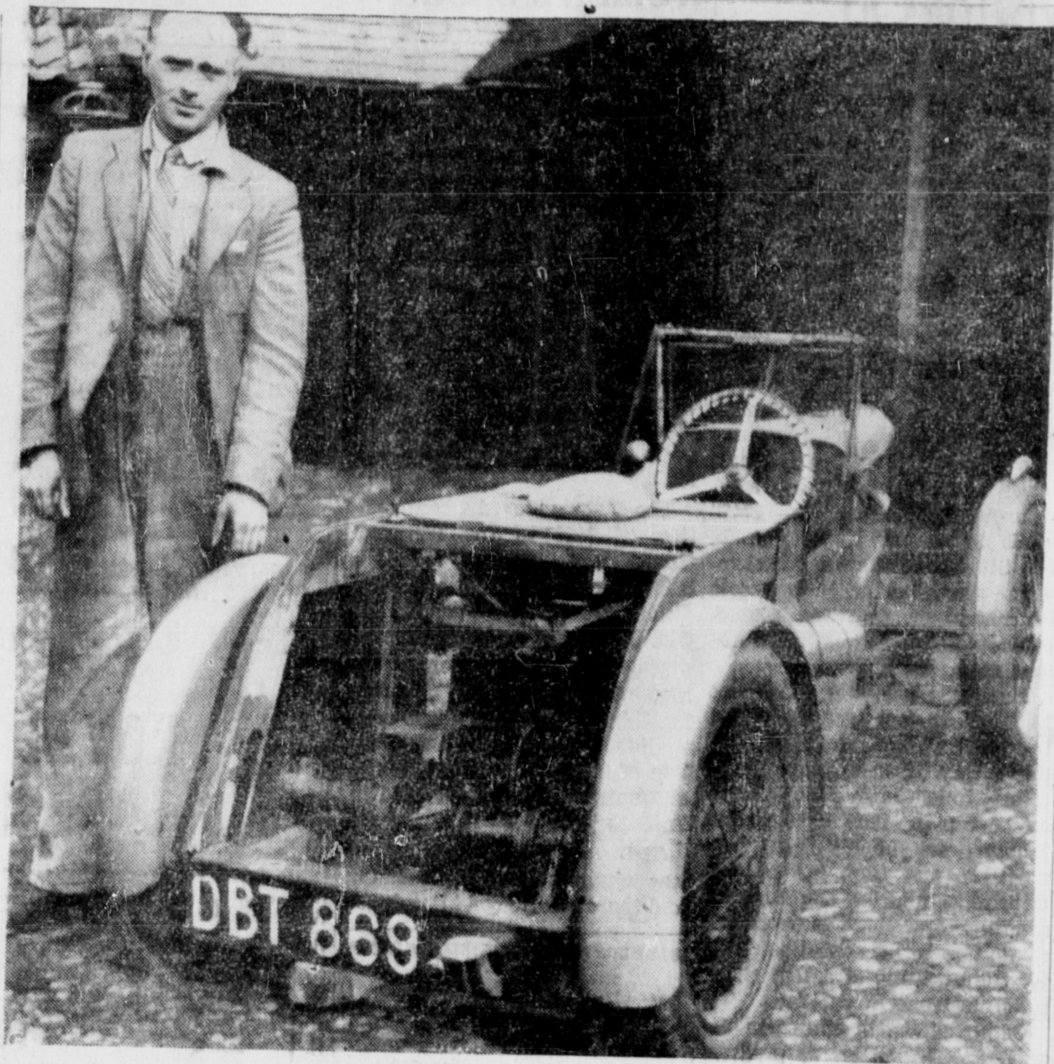
HOME-MADE CAR DOES 70 MILES TO GALLON—Jack McGrath, of Lowestoft, England, is shown with the 2½ h.p. car which he built himself. It does 70 miles to the gallon and could be mass produced, says McGrath, for £100 ($450). A 180-mile test run was trouble-free, but took seven hours because curious crowds held up the car at every halt.
