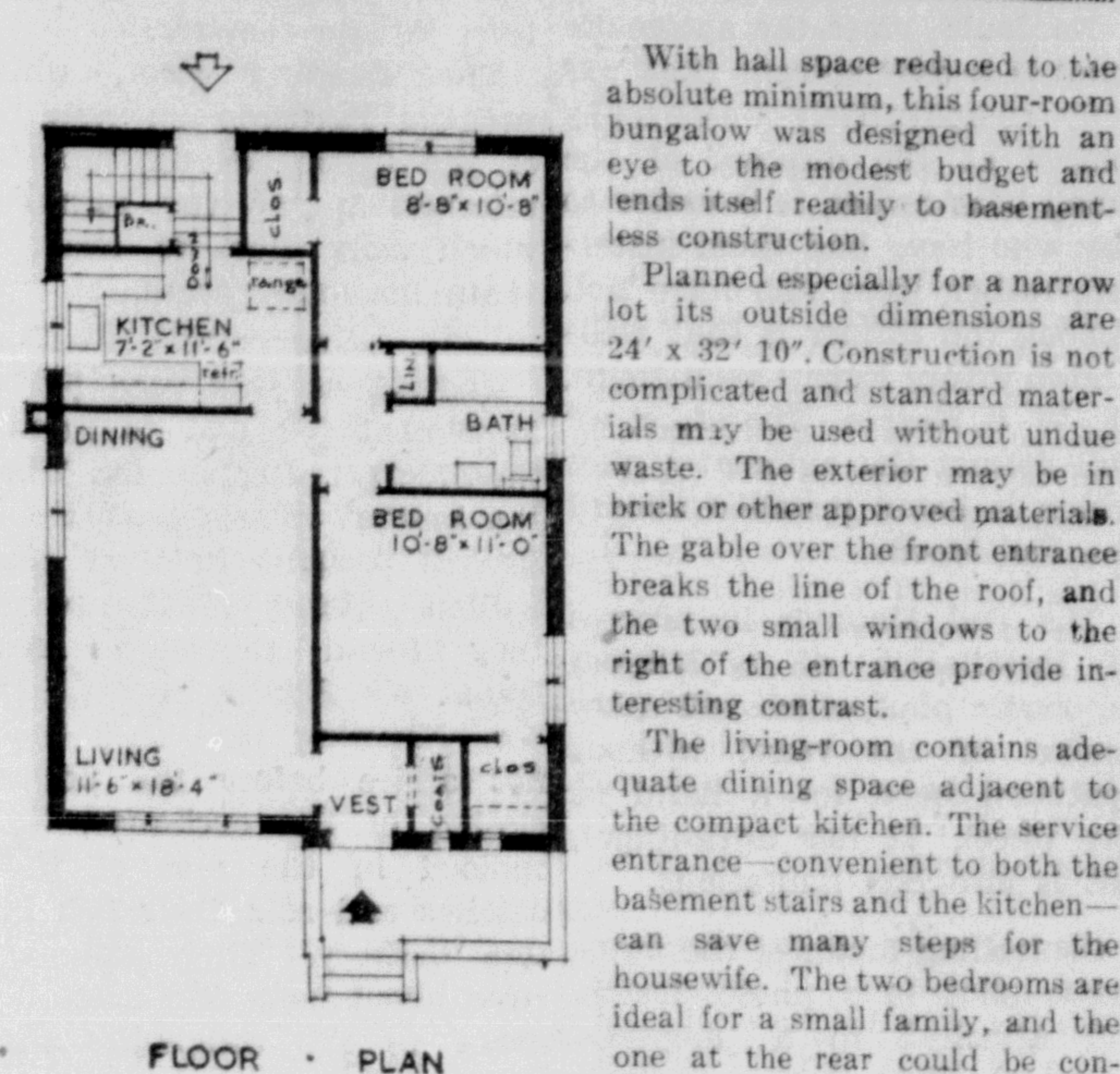
FLOOR PLAN The floor area, for estimating purposes, is 780 square feet.
