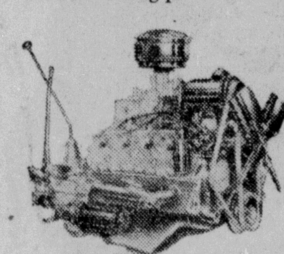
106-HP. V-8 TRUCK ENGINE 194 Ft. Lbs. Torque Series F-1 to F-6
