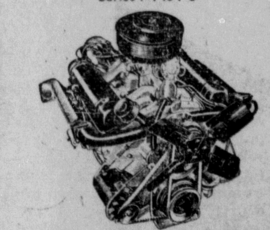
145-HP. V-8 "Cargo-King" ENGINE 244 Ft. Lbs. Torque Series F-7
