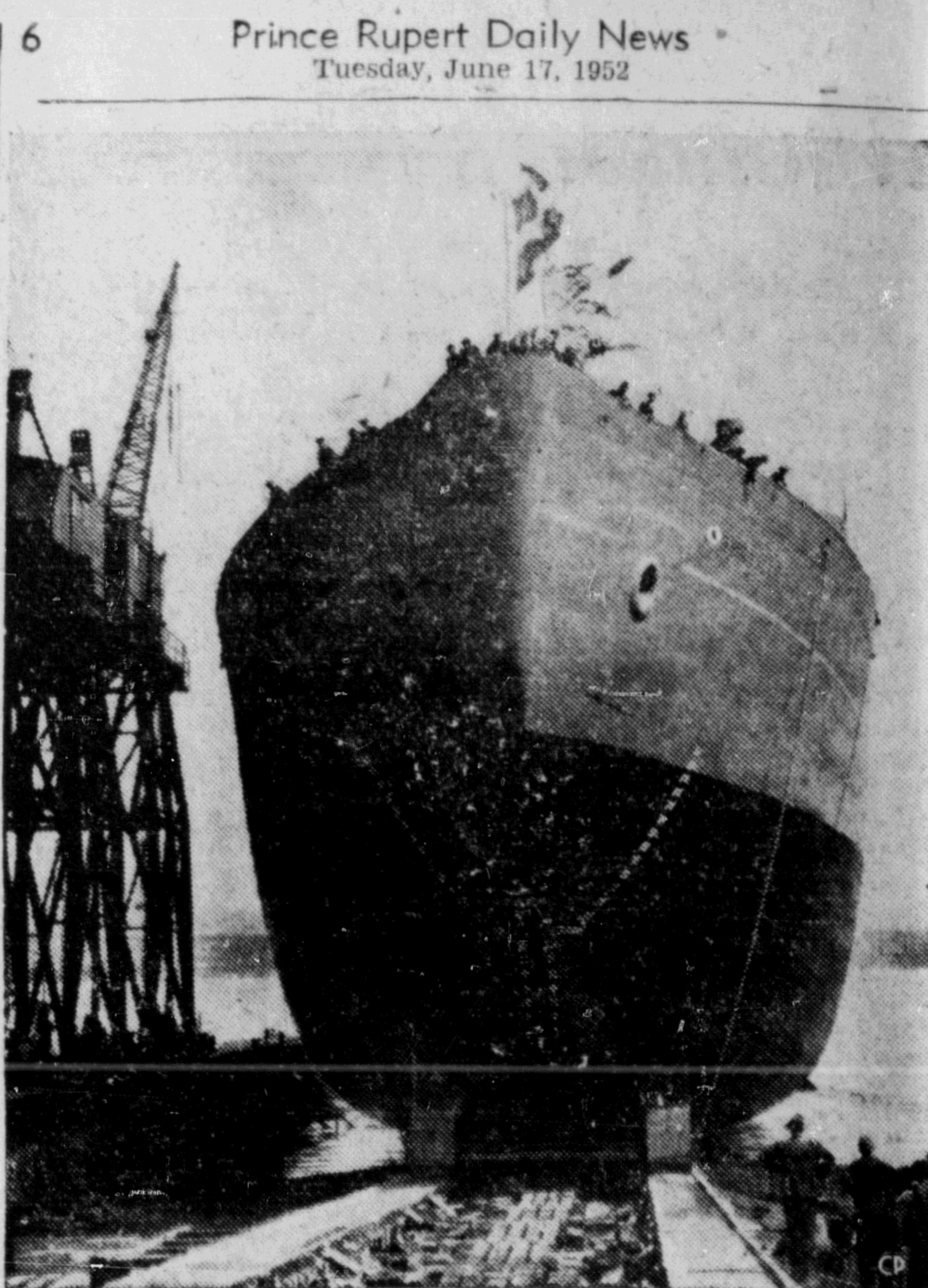
LARGEST ICE-BREAKER —The 3,100-ton hull of the d'Iberville, the continent's largest ice-breaker, slips into the St. Lawrence river at Lauzon, Que., where it was built. The Transport Department's new ship is able to cruise 12,000 miles without refueling and is expected to reach Arctic regions where no previous Canadian ships have touched. The d'Iberville will be equipped with two helicopters for photography and scouting. (CP PHOTO)
