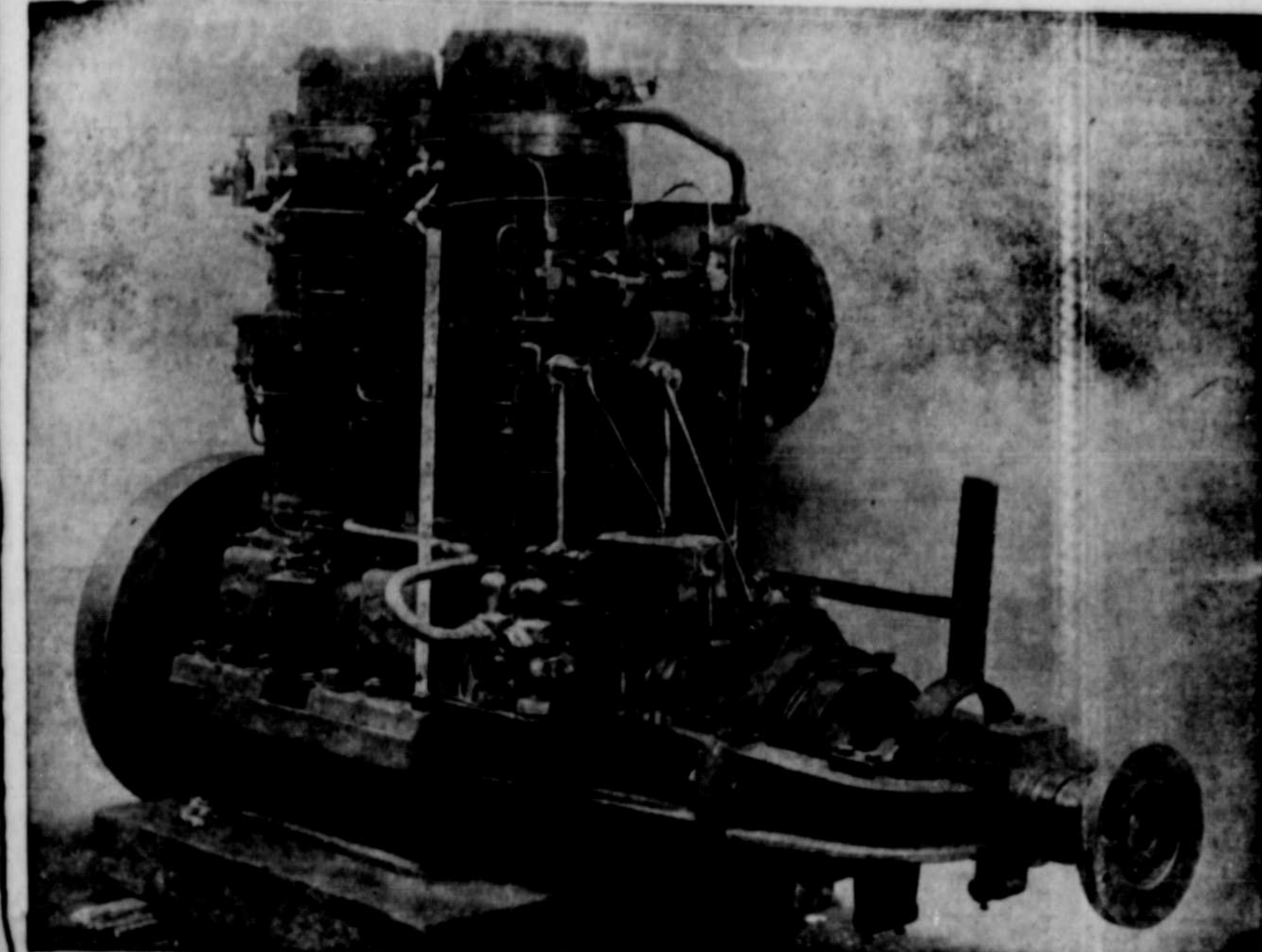
2-cylinder British Kromhout Engine, 50 H. P.
