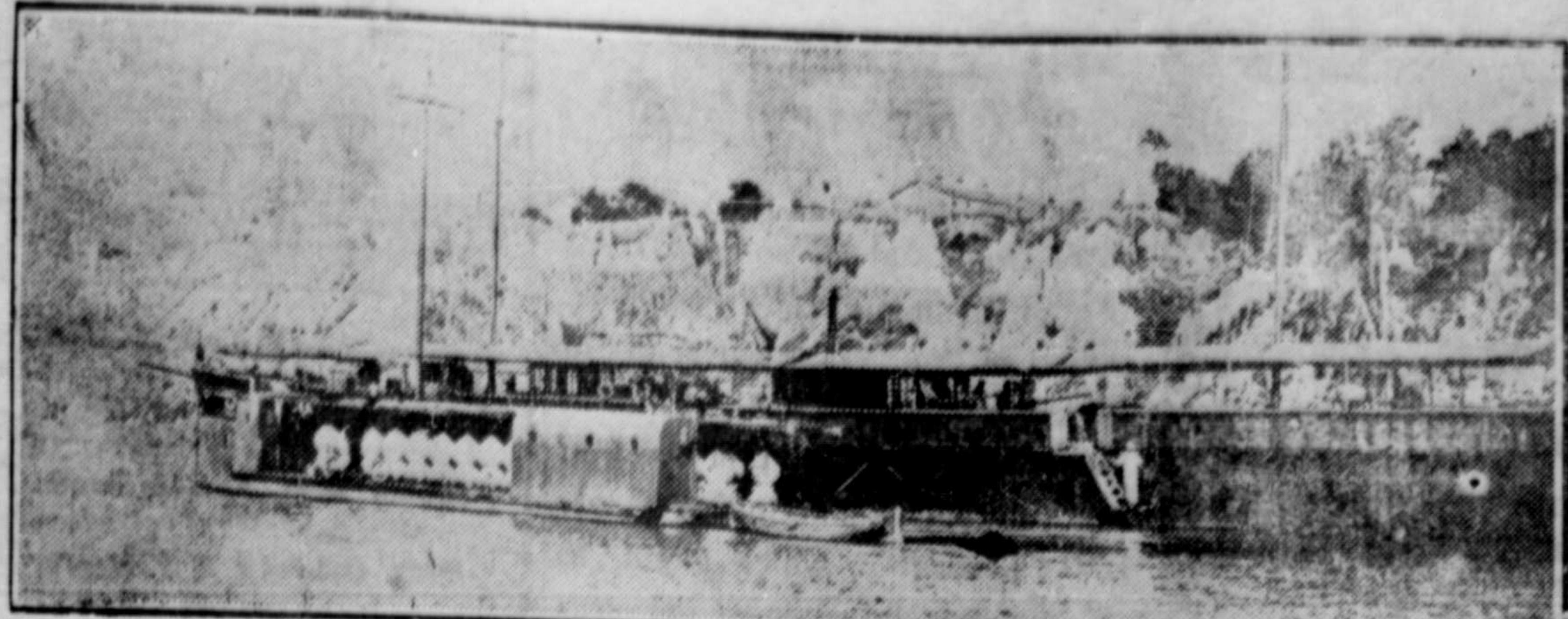
ROUMANIA READY FOR WAR. A Roumanian mine laying ship in the Danube. The mines shown in the picture are on rails and can be dropped over the stern and anchored at the desired point with ease.
