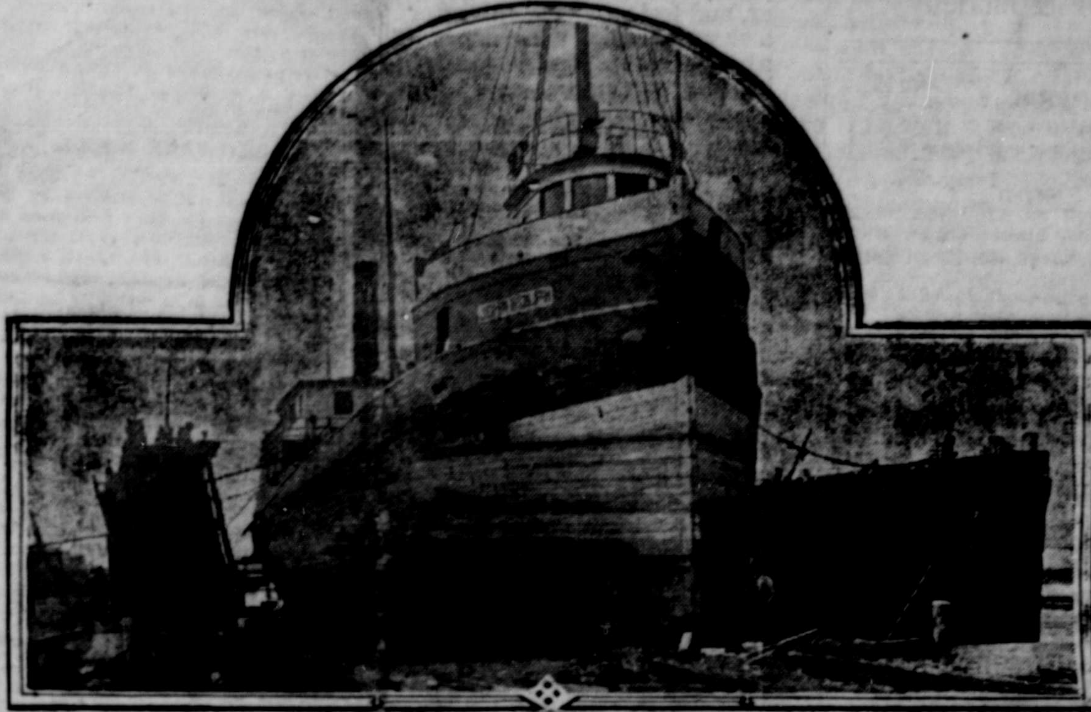
TORONTO HAS A NEW DRYDOCK. —This photograph shows the first ship drydocked for repairs in the new Toronto Drydock Company's plant. This is the first drydock of its kind in Toronto and was built in three sections, each section being 65 feet wide. The sections were brought across the lake from Sturgeon Bay, Wis.
