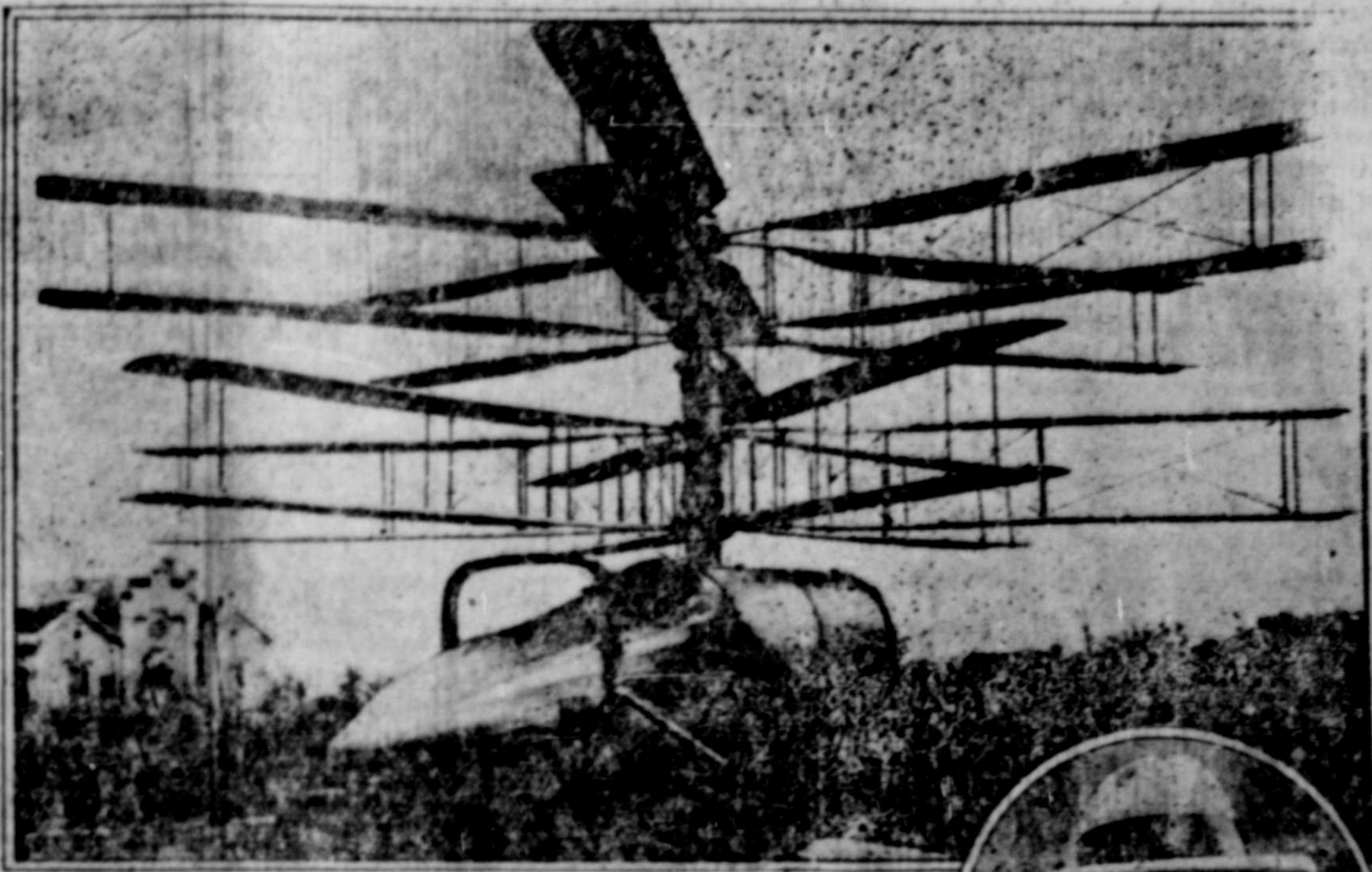
The Pescara helicopter, the latest machine of its kind in the world, has achieved vertical ascent in its preliminary tests at Buena Vista, the estate of Marquis Pescara. The helicopter made ten successful flights, each time rising about a yard, remaining aloft, maintaining perfect stability and then settling vertically to the ground. The preliminary trials put the new machine in line for honors in development of the helicopter. Marquis Pescara (in insert), a Spanish nobleman, is the inventor and is working in conjunction with French army engineers.
