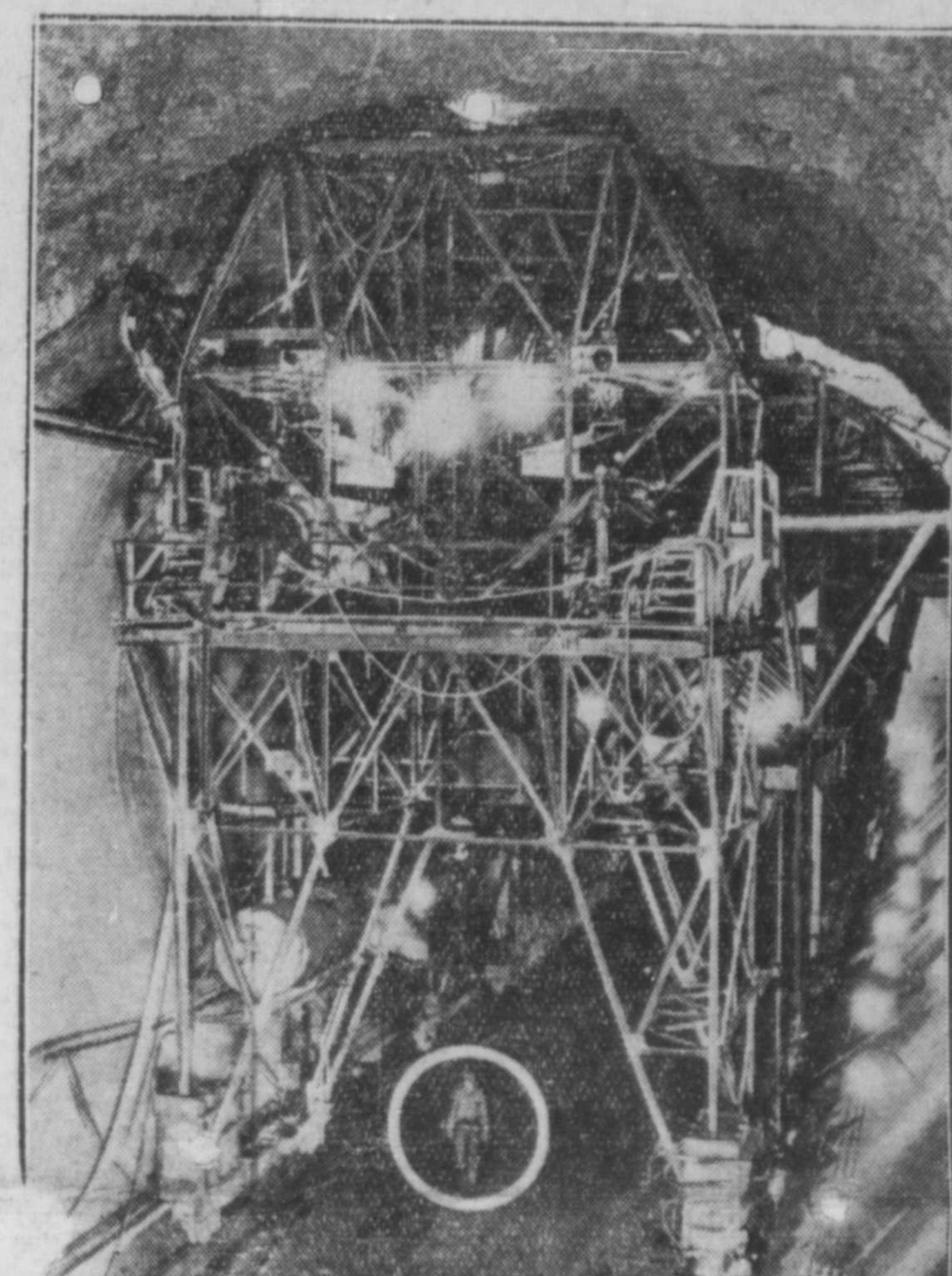
This compressed air concrete gun carriage is placing 110 degree top arch concrete in the diversion tunnel of Hoover dam at Las Vegas, Nevada. Material is brought to the job in dump trucks. Note size of workman.
