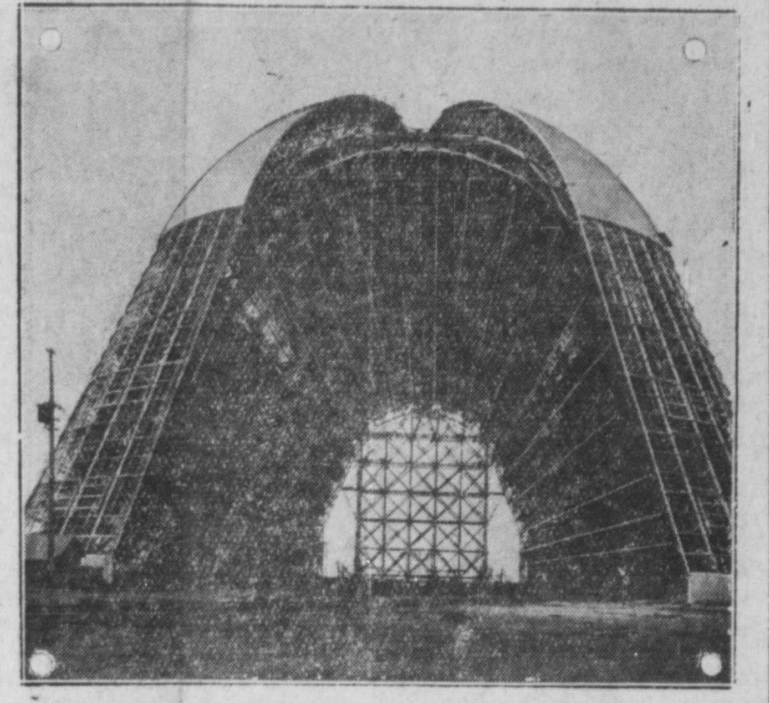
The second largest hangar in the world, a mammoth structure, 1,138 feet long, 310 feet wide and 198 feet high is nearing completion at Sunnyvale, California. It will cost about $1,697,000.
