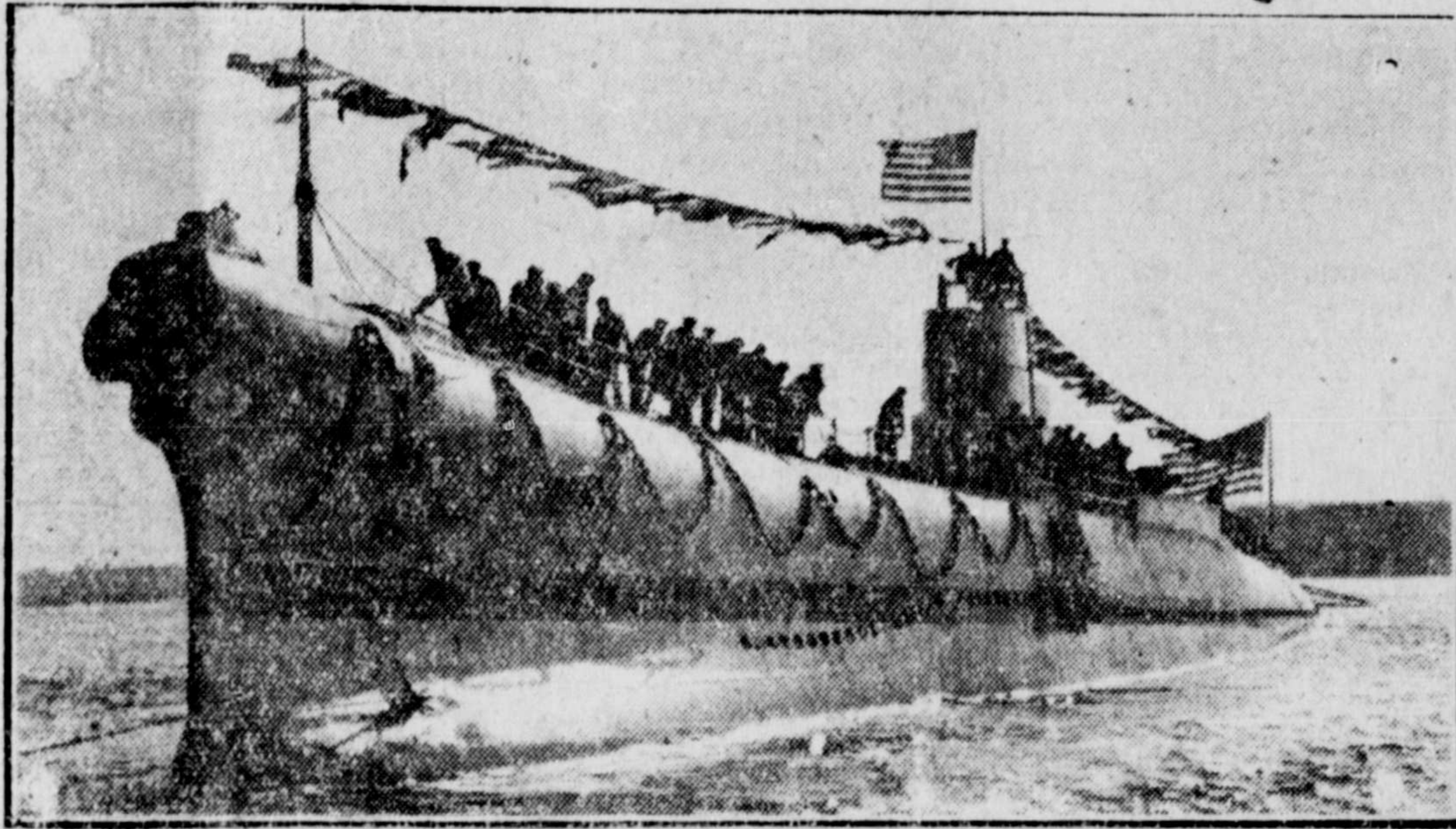
The new United States submarine U.S.S. V-2, which was recently launched, has a surface speed of 21 knots and a submerged speed of 9 knots. The vessel carries six 21-inch torpedo tubes.
