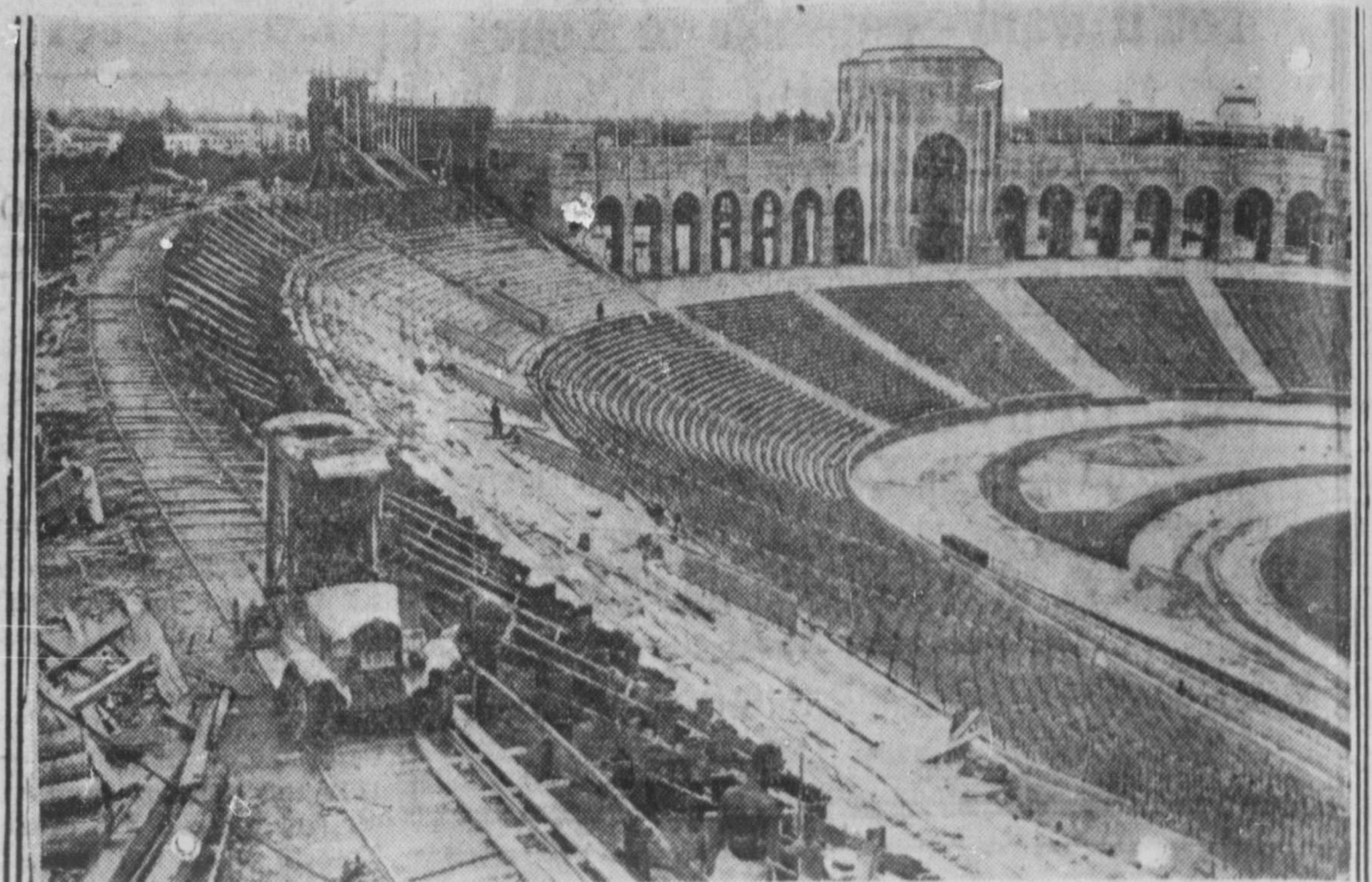
Thousands of tons of concrete are poured into famous Los Angeles coliseum, where most of track and field sports will be held in 10th Olympic games.
