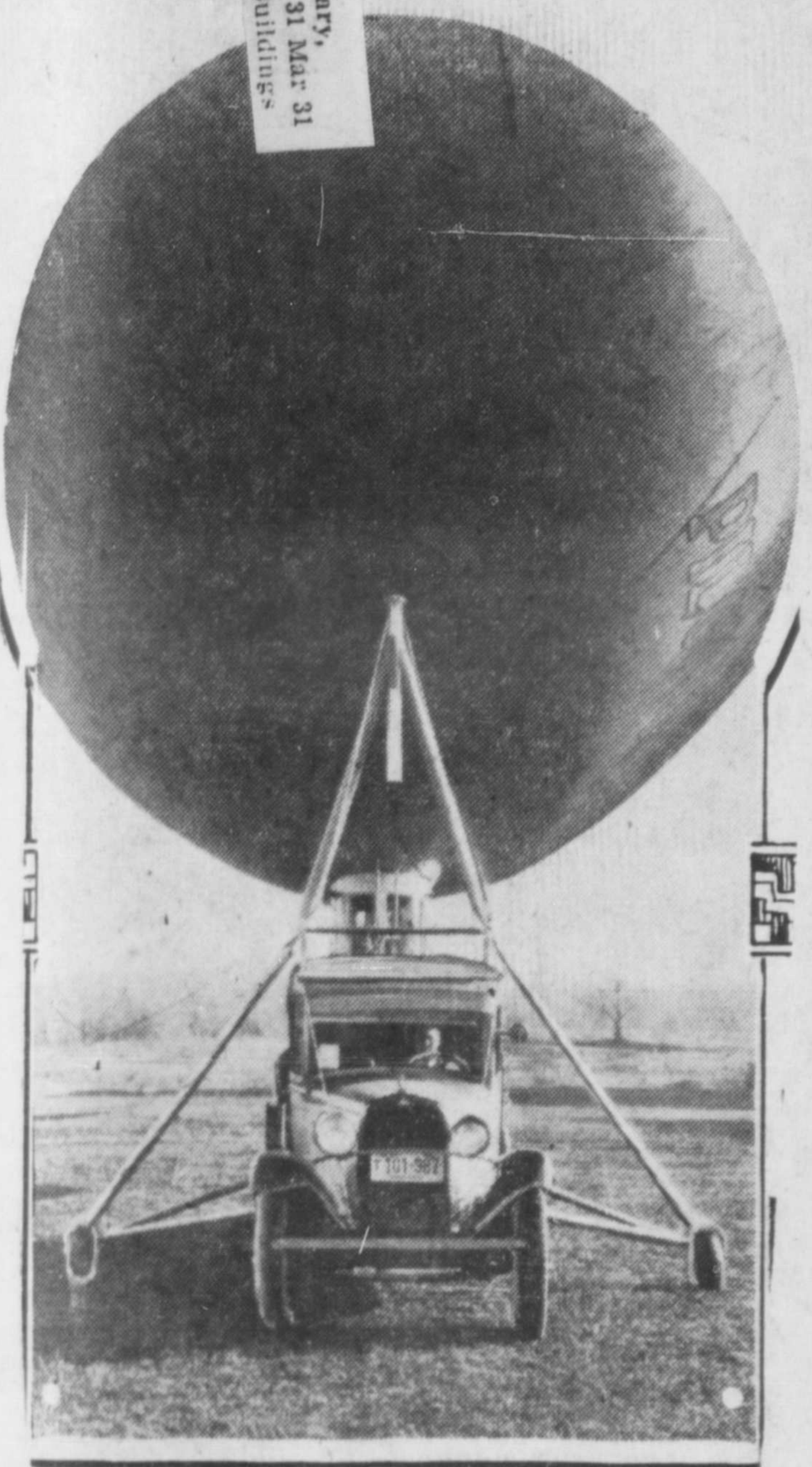
New portable mooring mast or travelling harbor can be folded and clamped down to roof of bus when not in use. Outrigging prevents bus from tipping in case a heavy wind strikes ship. Car is also used to transport ground crews.
