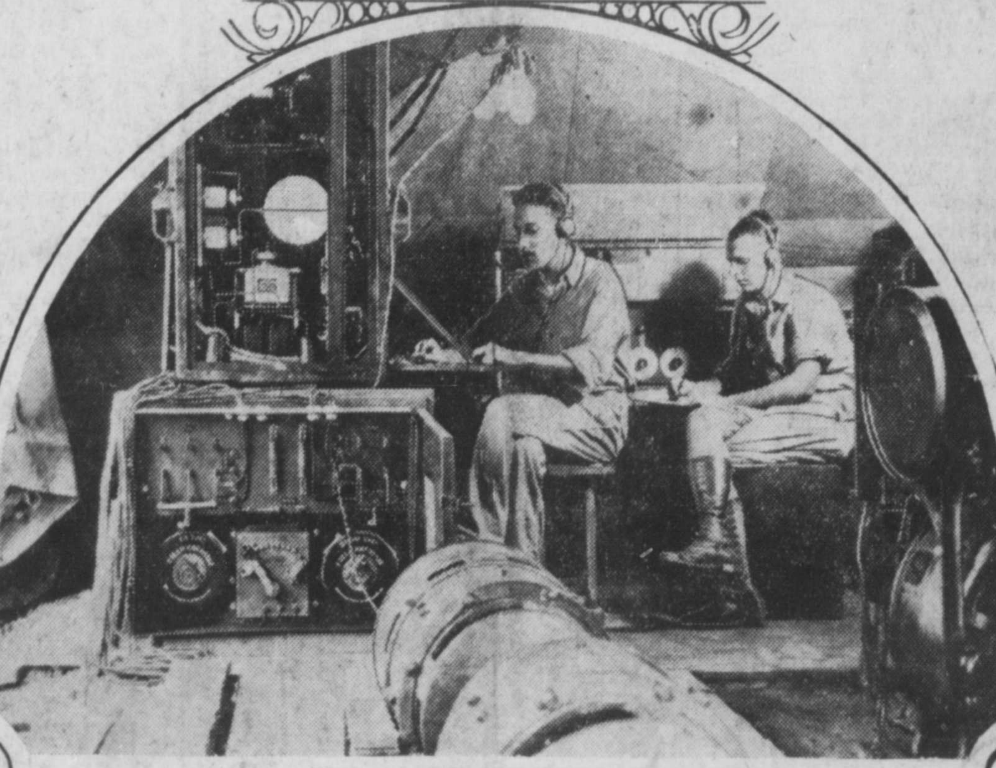
Central wireless installation set used to maintain communication between headquarters and field forces on journeys by canoe or oxcart in Nicaraguan jungle on new American canal construction here
