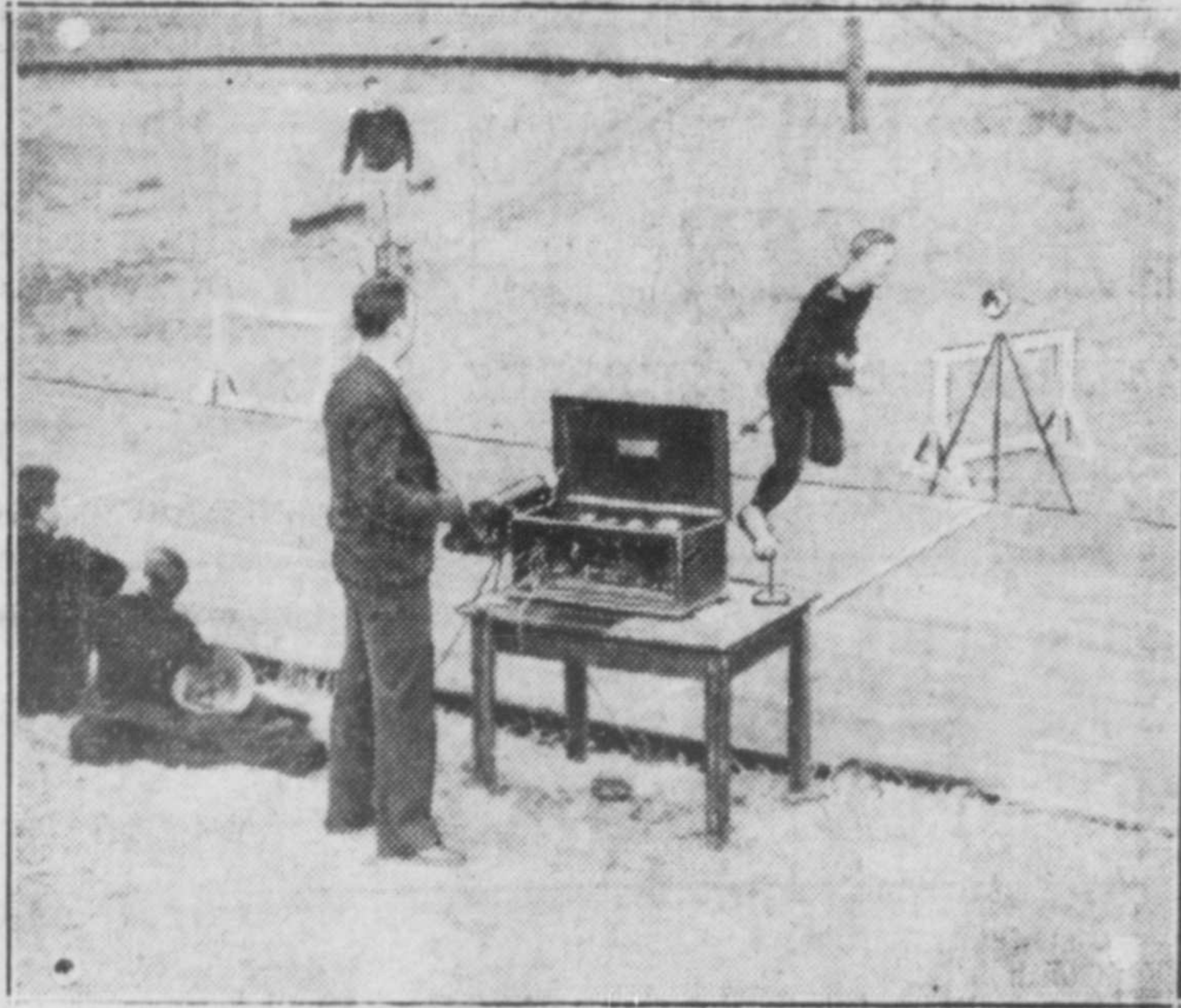
Haverford college students crossing finish line of new racing ray constructed by Edwin Speakman of Haverford, which projects a beam of light across race track, registering running time to one one hundredth of second
