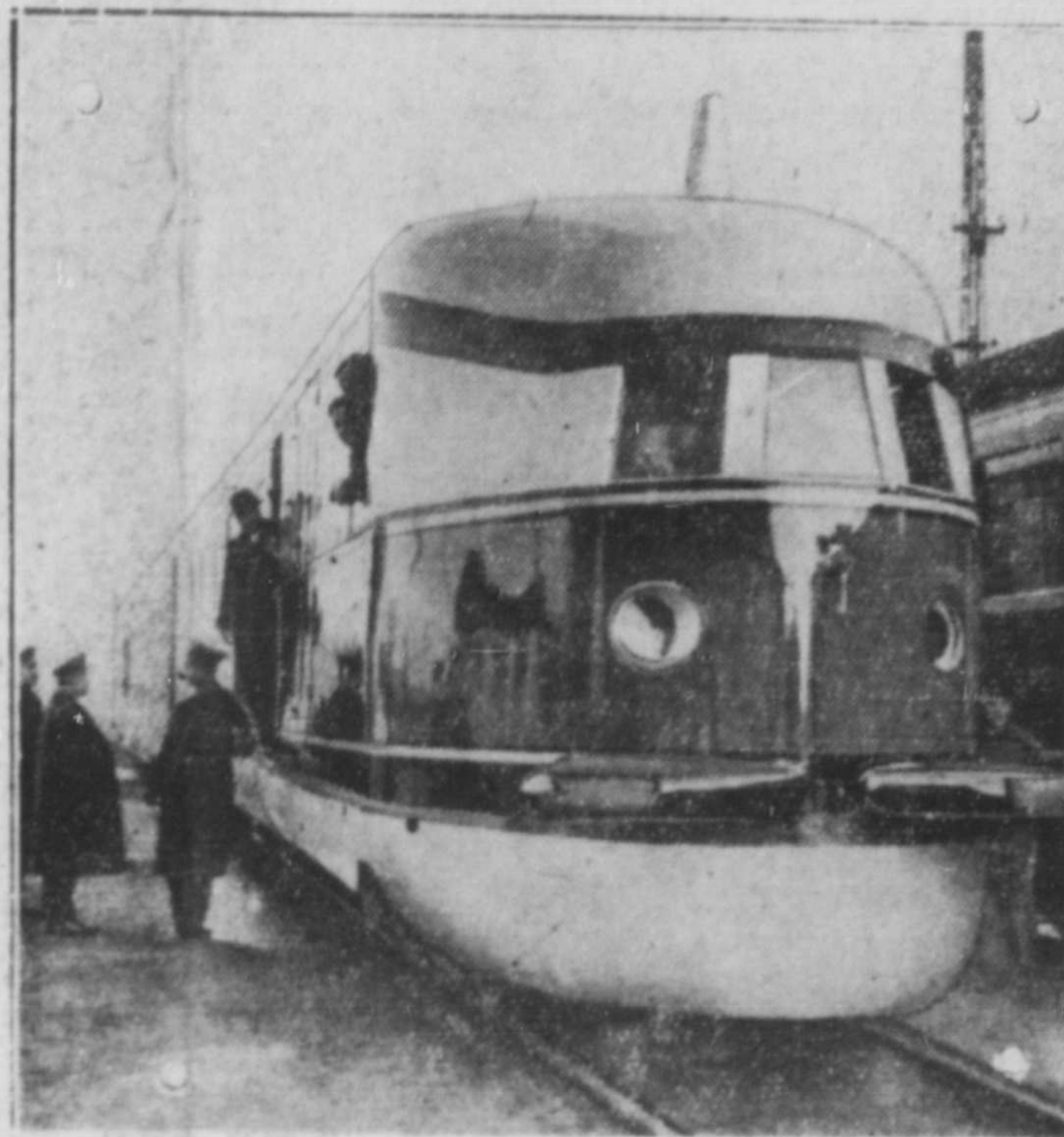
If you want to get anywhere fast try a trip in the "Flying Hamburger," world's fastest train, which zips from Berlin to Hamburg and back at 95 miles an hour. A 419 h.p. Maybach engine supplies the pep.
