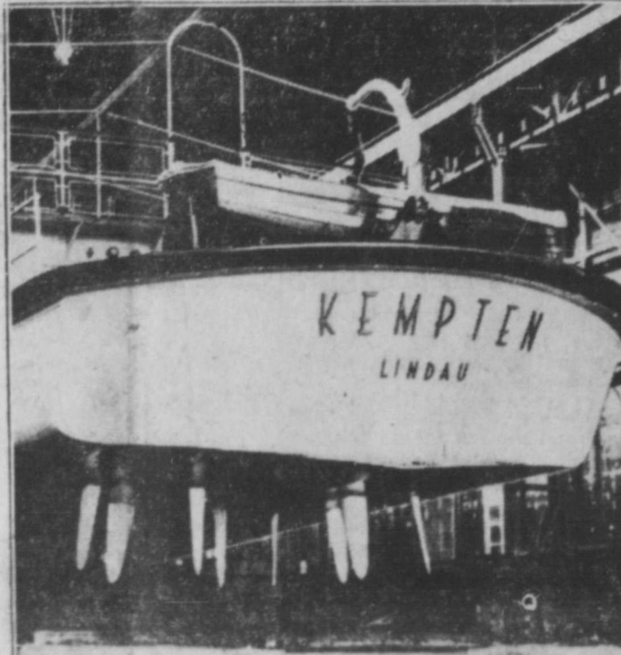
Combination propeller and rudder. This strange device is used by a German firm for traffic on Lake Constance. It consists of a runner rotating around a vertical axis equipped with four mobile blades which also steer the craft.
