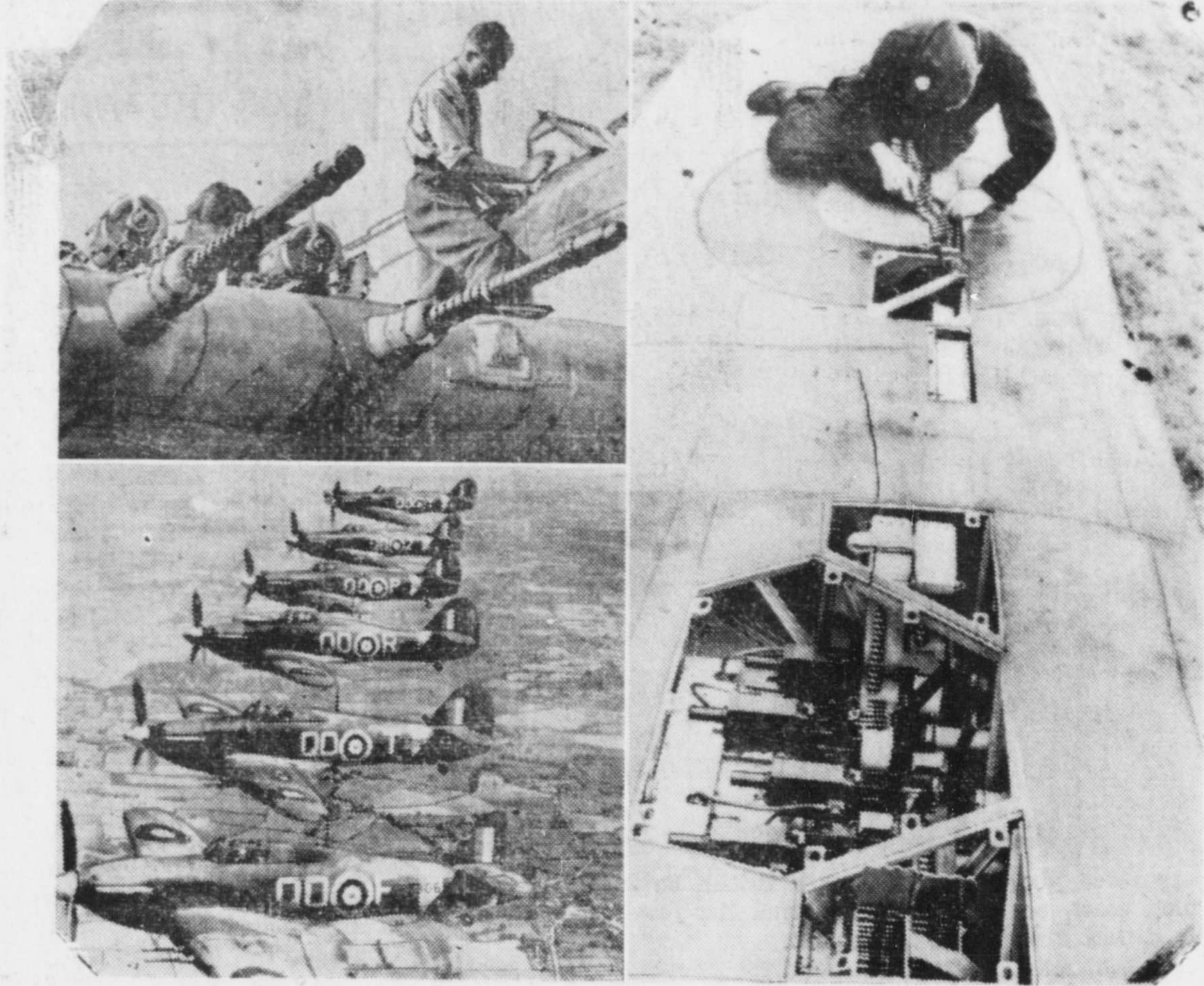
Three pictures which illustrate the new Hurricane II, the fighting plane which the Royal Air Force recently introduced as an improvement over the Hurricane I. The new planes are fitted with Merlin engines, but most important of all, their armament has been vastly increased. One group of Hurricane II's are fitted with 12 machine-guns, the second group having four 20MM cannon mounted in the forward edges of the wings. At the top, left, is a closeup view of two of the powerful cannon as mechanics put the plane in shape for combat duty against the Nazis. Below, left, a squadron of Hurricane II's, equipped with the four cannon, is shown in flight. At the right is a rare picture made from the plane cockpit, showing cartridge belts being fed to some of the 12 machine-guns with which the plane is fitted.
