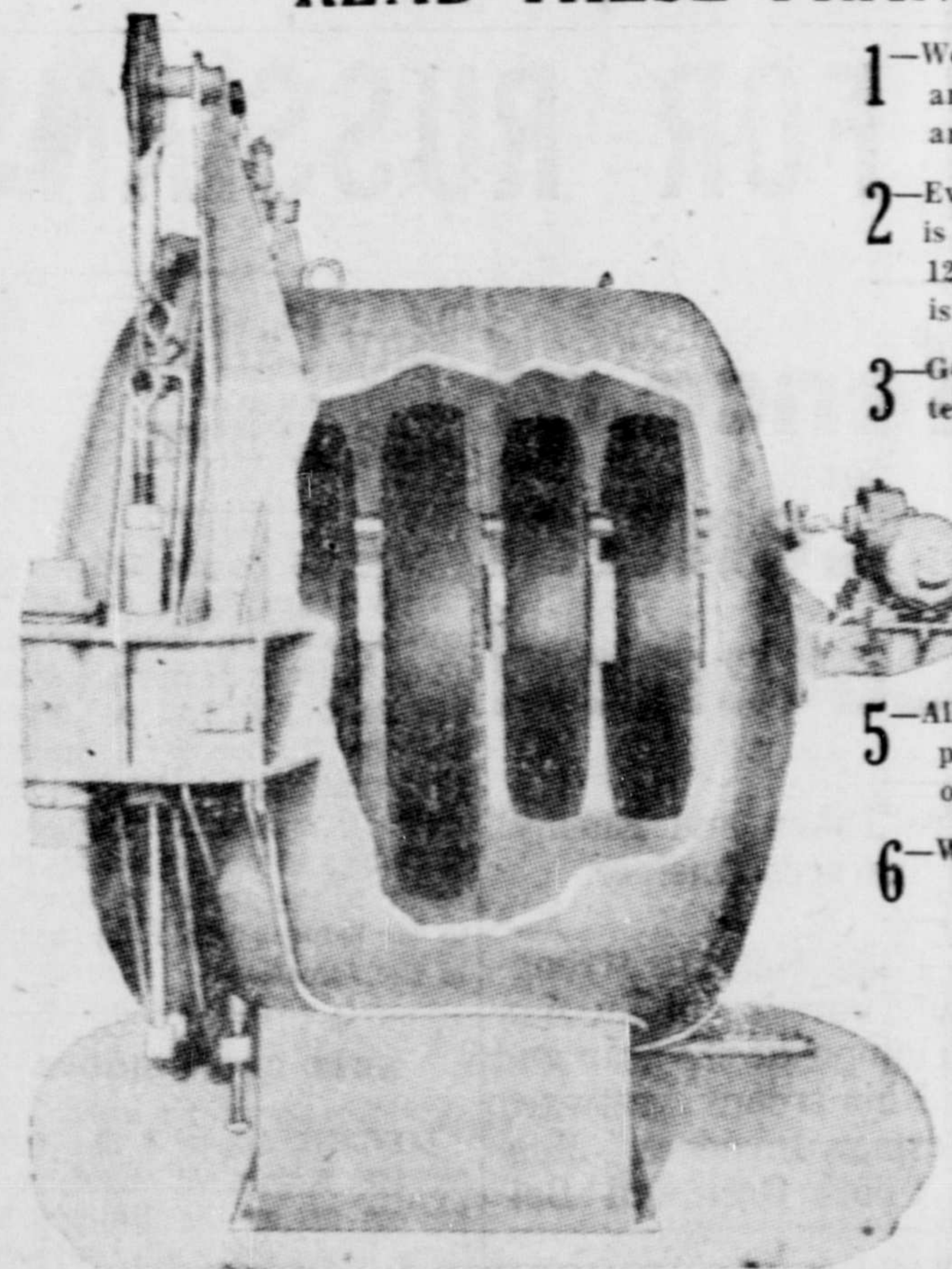
Illustration shows the "VITACAP" recapping machine in action. Tires are rotated in the curing chamber so that live steam is applied to all sides of the casing. Result is uniform tread rubber hardness at both surface and base. "VITACAP" is the finest recapping and vulcanizing process in use today.
